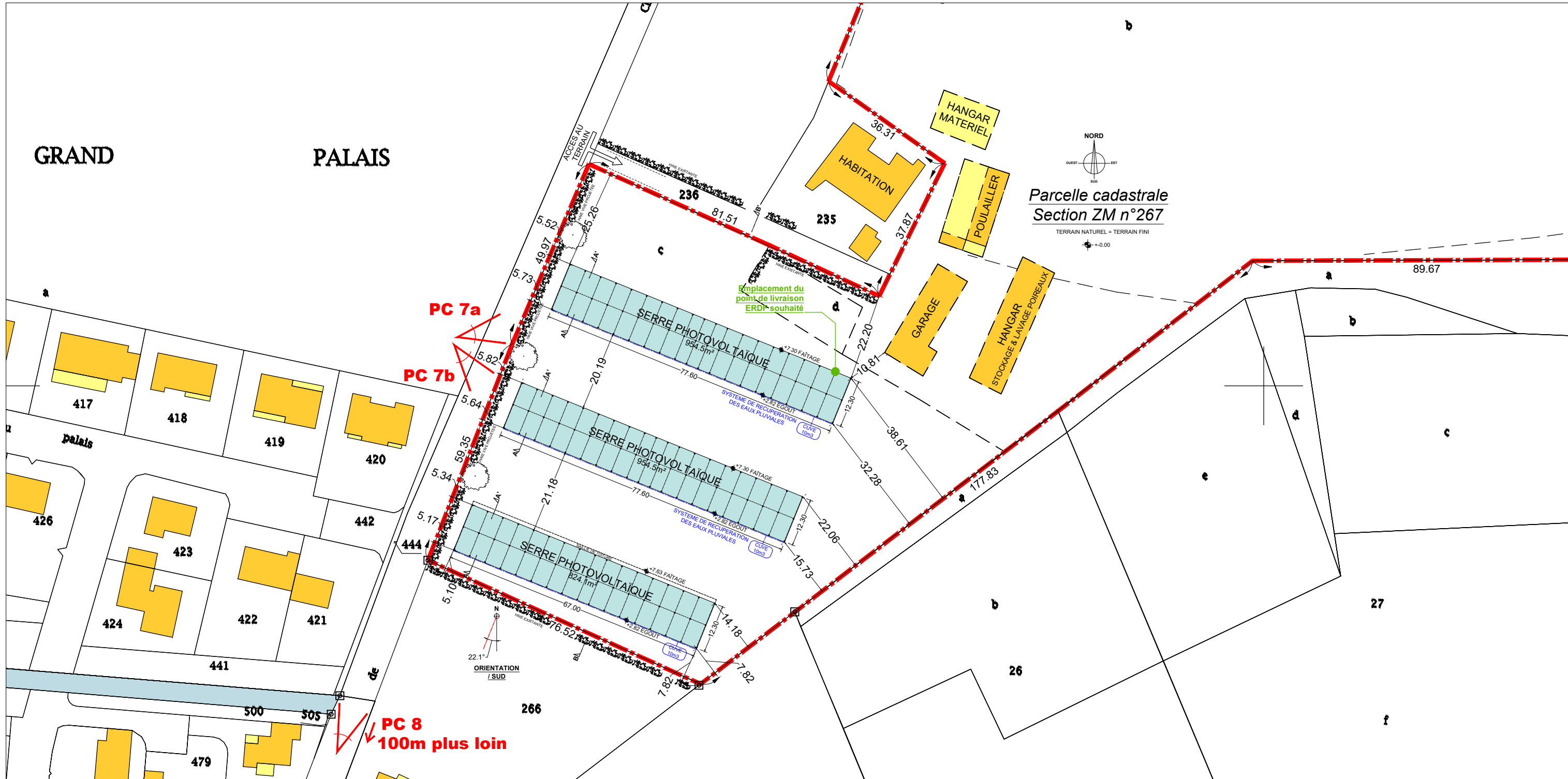
PC2_PLAN MASSE - 1 / 1000
